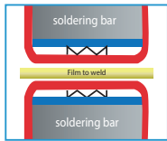
Impulse welding Jaws equipped with welding wires
