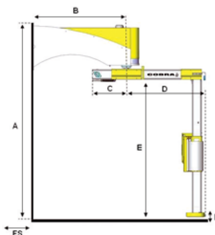
The Power Pre Stretch carriage is driven by belt lift and pre stretch wheels are easy to remove and change.
